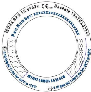
Fig. 1 Identification label 1
